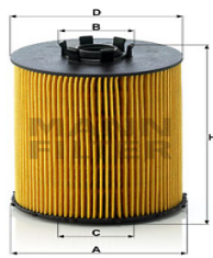
Oil Filter HU 823 x EM-10045
