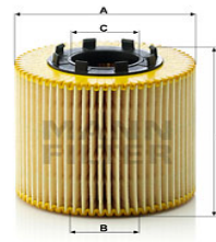
Oil Filter HU 923 x EM-10183
